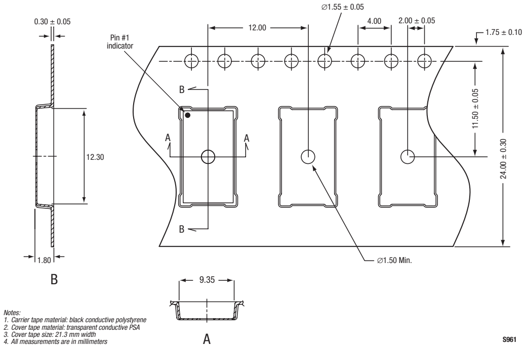
Figure 9. SKY73101 Tape and Reel Dimensions
