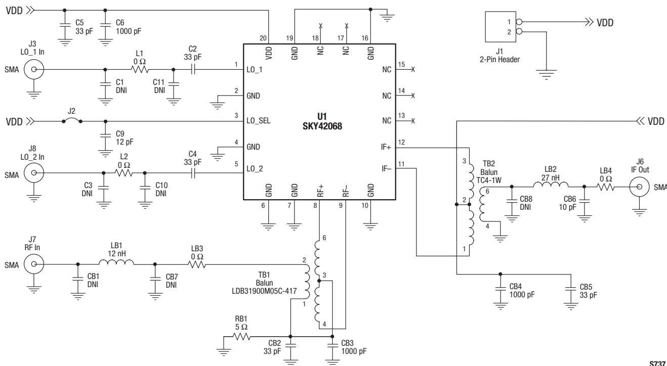
Figure 3. SKY42068 Evaluation Board Schematic (900 MHz)
